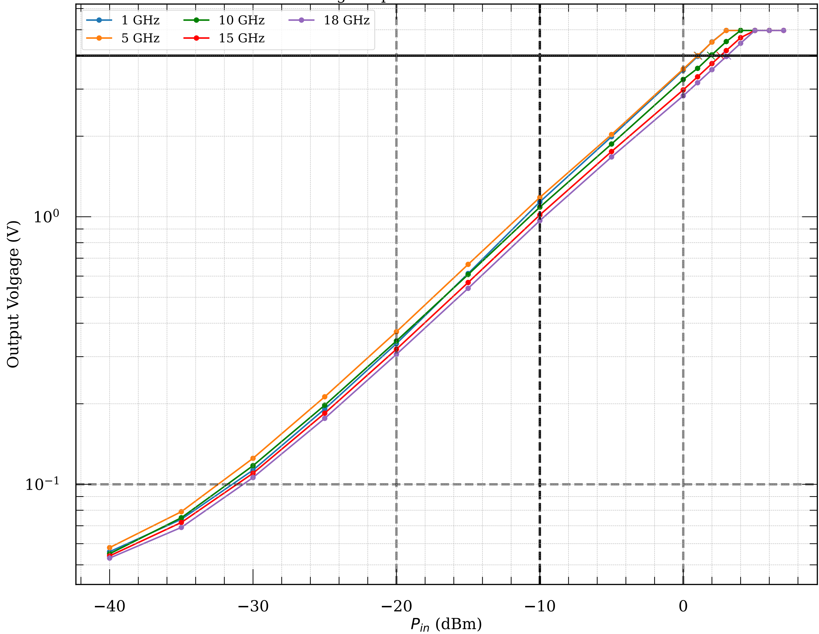
Measured voltage-to-power curve of detector module020v2
